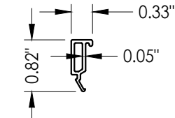
6 GLAZING BEAD Extruded vinyl
